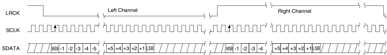
Figure 30. Format 1, I²S
