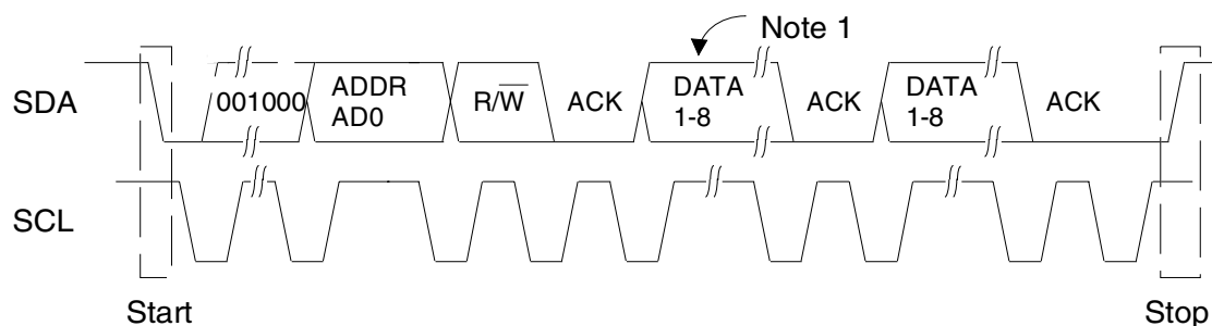
Figure 8. Control Port Timing, I²C Mode
