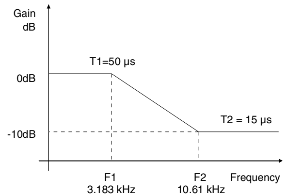
Figure 28. De-Emphasis Curve
